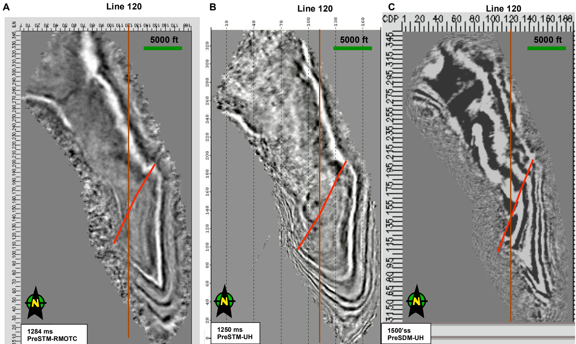
Figure 12. Seismic time and depth slices near top granite basement extracted from UH processed and commercially processed (RMOTC data) prestack time migrated volumes and a UH processed prestack depth migrated volume. A. 1284 ms time slice from RMOTC seismic volume. B. 1250 ms time slice from UH seismic volume. C. 1500 subsea depth slice from UH seismic volume. Faults: red. Because of different seismic processing datums, TWT values are not exactly correlative between UH and RMOTC volumes. See Figure 2 for seismic section along Line 120 and locations of slices.
