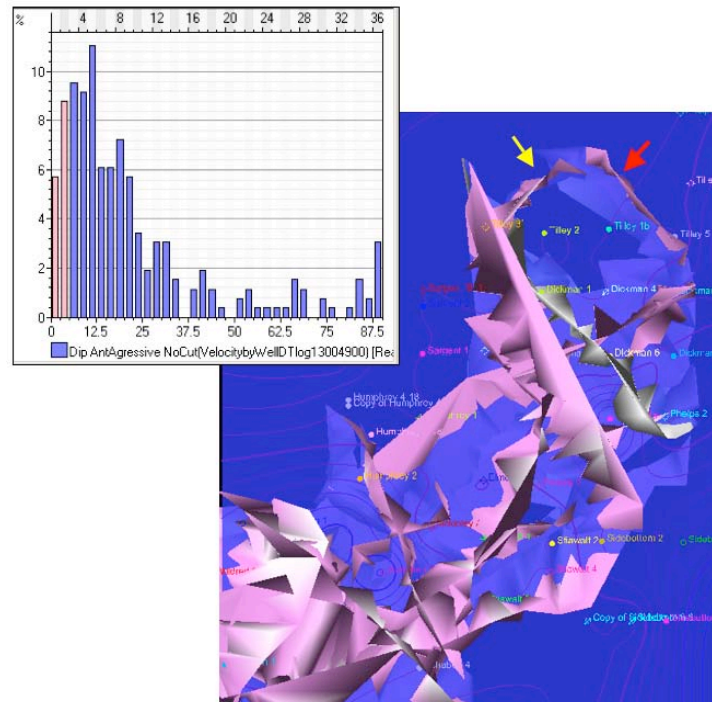
Figure 1-6b. Selected Planes Extracted from the Aggressive ANT Volume. All planes with dips > 5^\circ are shown by the blue bars in the histogram to left. The NW plane (red arrow) is 4000 ft long and the NE plane (yellow arrow) is 2000 ft long. Scale is 1:1.
