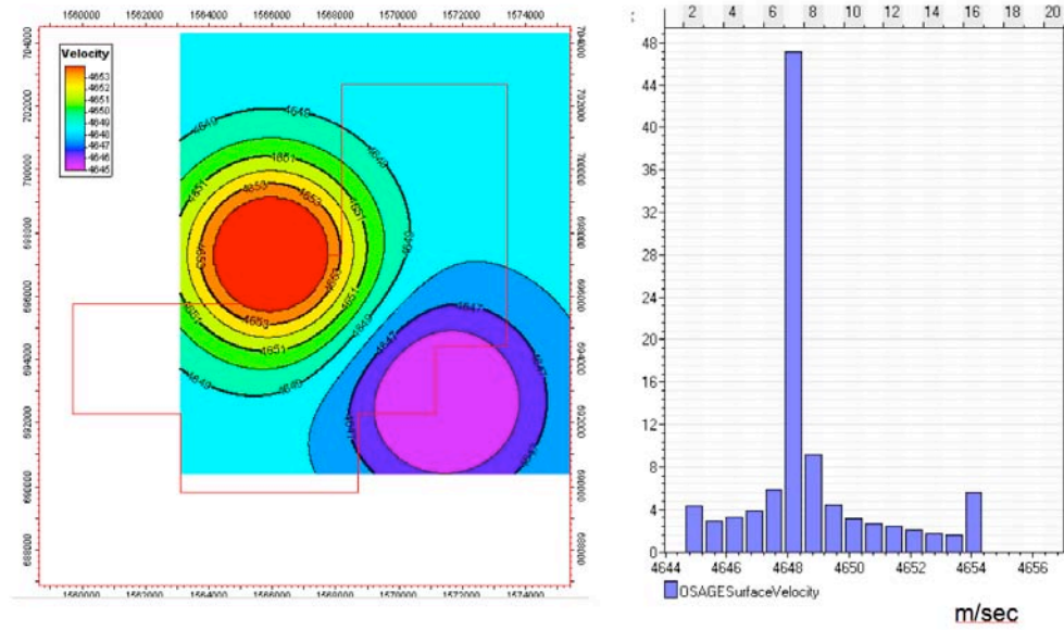
Figure 1-2d. Interval velocity distribution for Osage to Gilmore City (GMC). With only 2 control points, values range from 4646-4654m/sec, and 50% at 4648 m/sec. Note the extreme low in Sidebottom 6. As an input set for building a velocity model, upper and lower 5-7% of the velocity extremes in the distribution are eliminated. The range used is from 4646-4654 m/sec.
