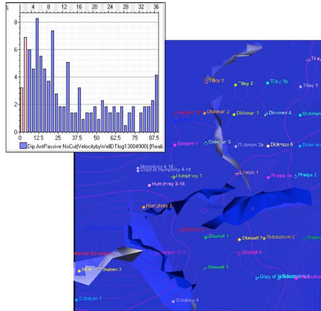
Figure 1-6a. Selected Planes Extracted from the Passive ANT Volume All planes with dips > 5^\circ are shown by the blue bars in the histogram to left. The blue surface to the right with contours is the OWC. Most of the extracted planes were eliminated by the five factors described in the text and therefore not shown. The Passive ANT revealed four NE features and two NW features. Scale is 1:1.
