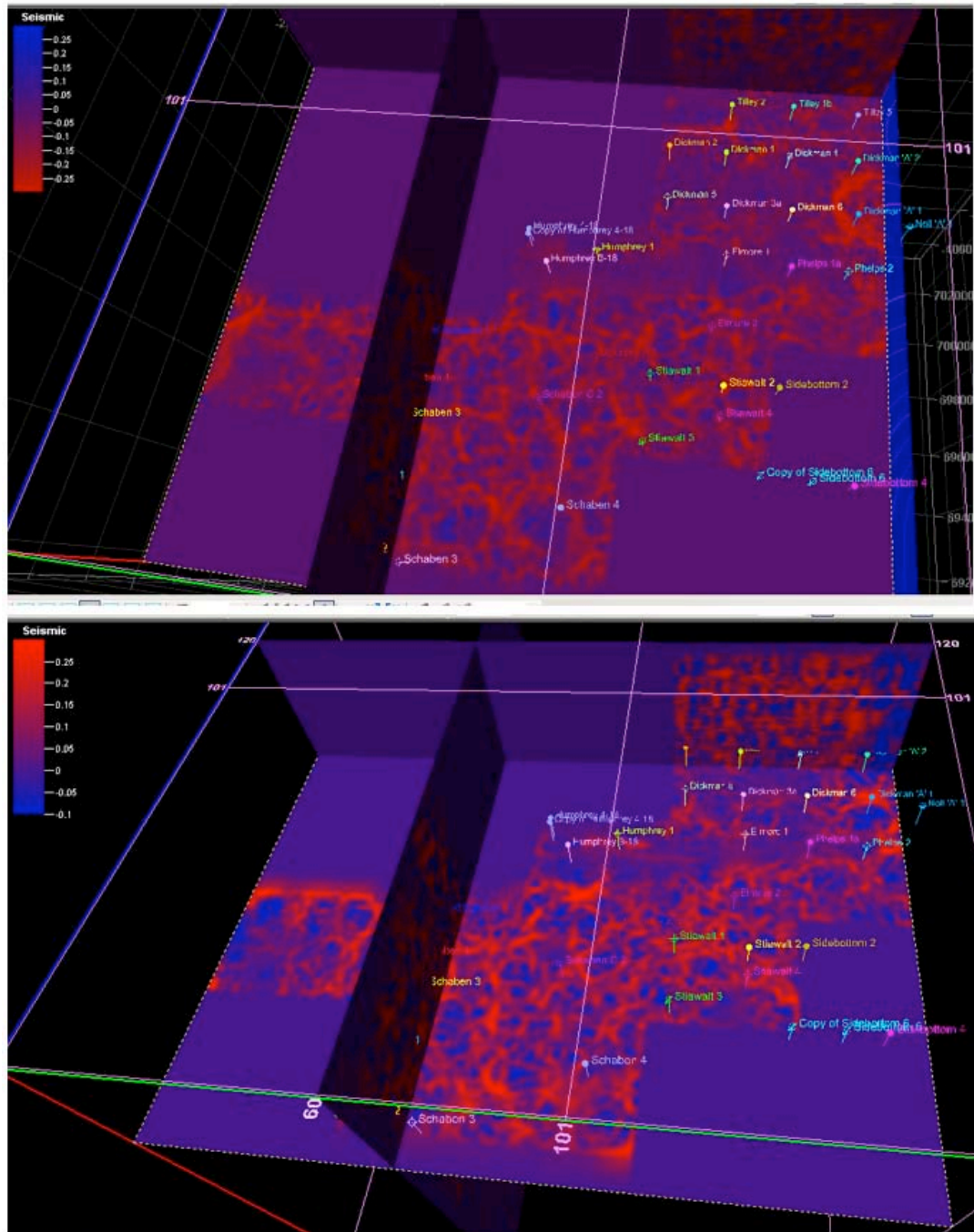
Figure 1-8b. Mississippian level curvature slices (-1960 TVDSS, about 15-20 ft above the OWC). Upper: Maximum negative curvature. Lower: Maximum positive curvature.
