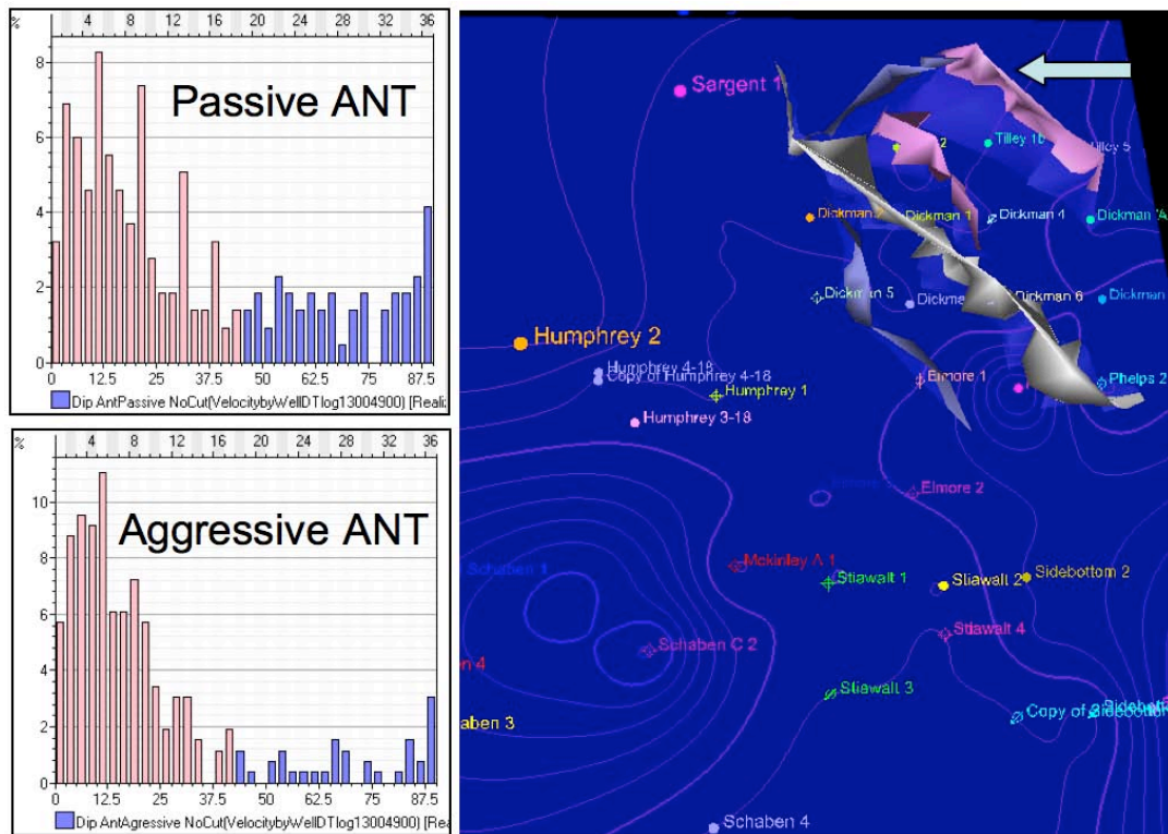
Figure 1-7b. Extracted ANT planes with dip > 45^\circ . One 4000 ft long NE plane (arrow) was extracted from both passive and aggressive ANT volumes.
