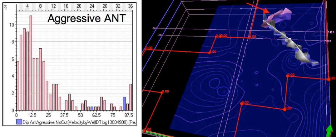
Figure 1-7a. Extracted ANT planes with dip > 60^\circ (vertical scale 1:1). Blue bars in the histogram correspond to the two planes shown. More than 80% of the planes extracted from the Passive ANT volume and more than 90% of the planes extracted from the Aggressive ANT volume are with dips less than 30^\circ . Length of NE Boundary Fault (red arrow) is about 2000 ft. OWC shown in blue.
